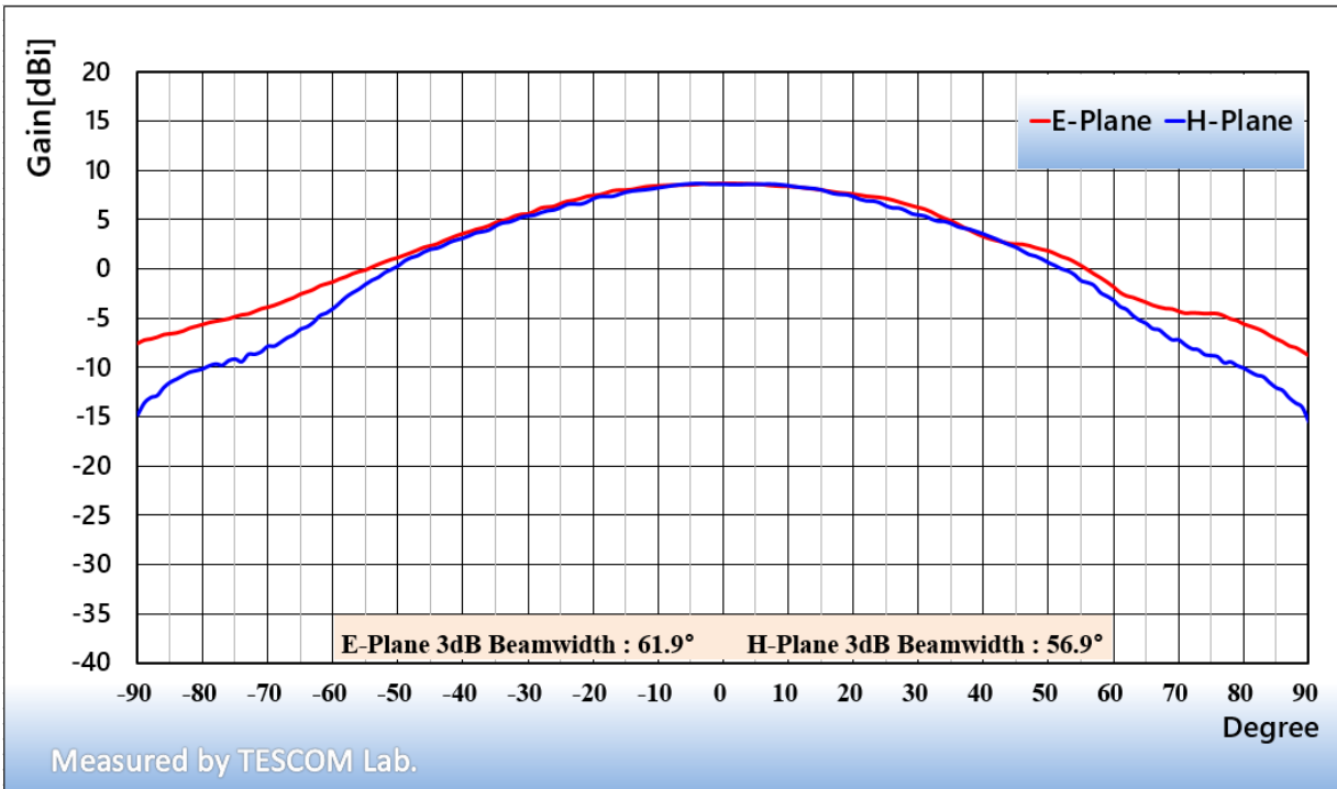
<TC-93473B @ 28 GHz>
