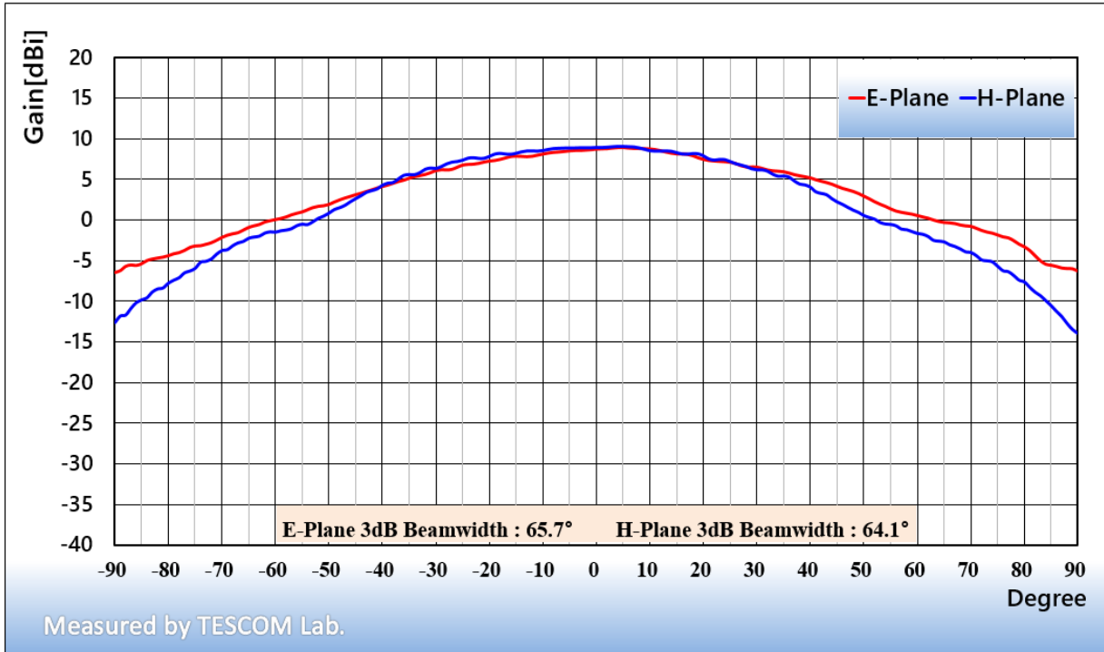
<TC-93473B @ 24 GHz>
